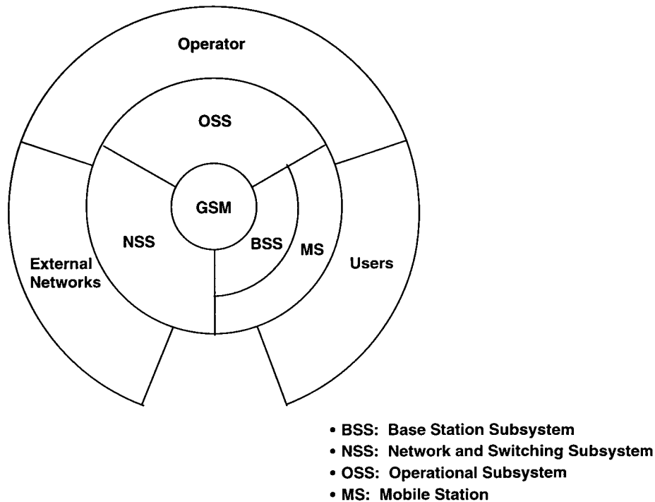
Fig. 5.2 GSM Subsystems
