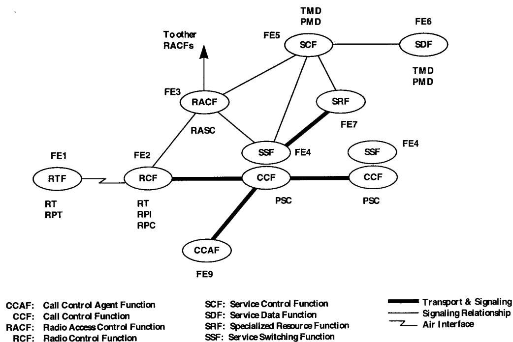
Fig. 5.8 Functional Model Derived from T1P1 Reference Model [1]
