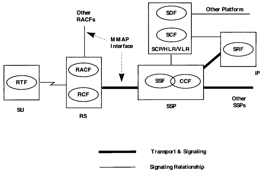
Fig. 5.9 Functional Entity Groupings
